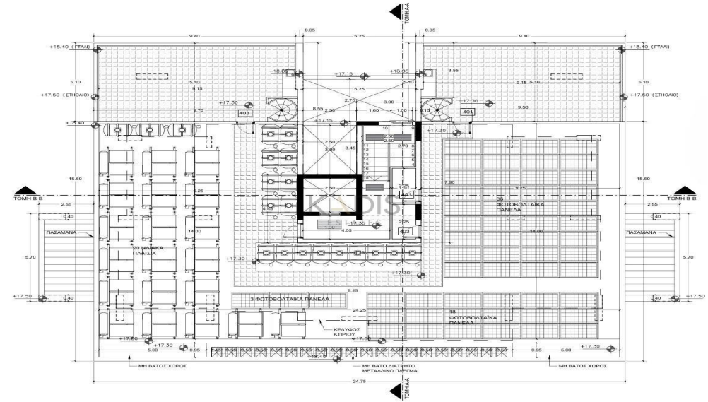
ROOF PLAN
