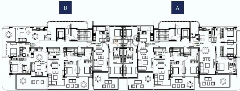
BUILDINGS A & B SECOND FLOOR
