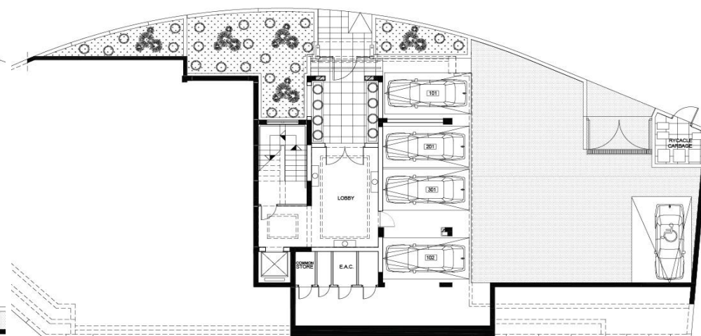
basement floor
