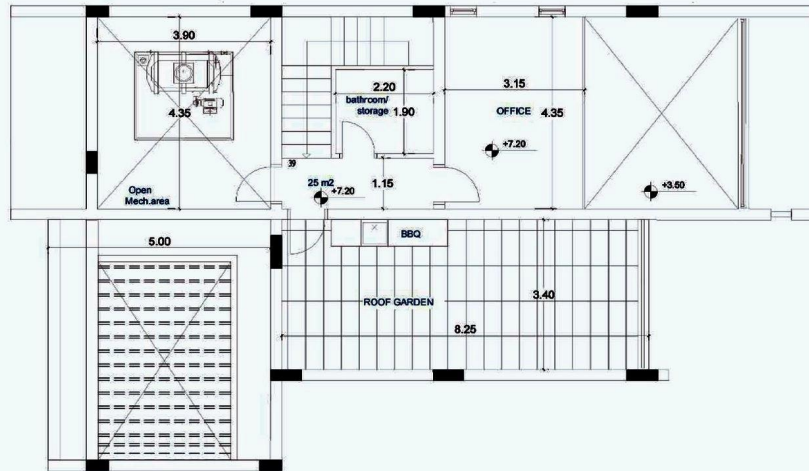
ROOF FLOOR
