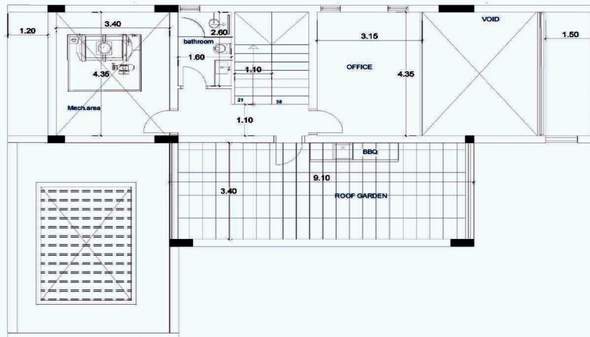
ROOF FLOOR
