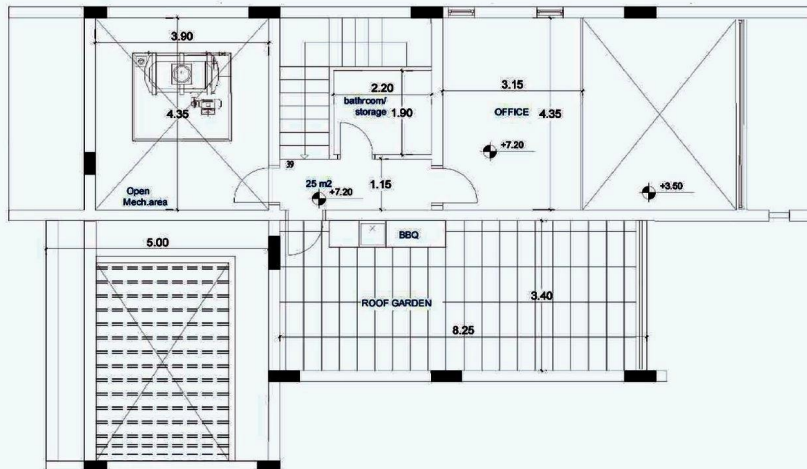
ROOF FLOOR
