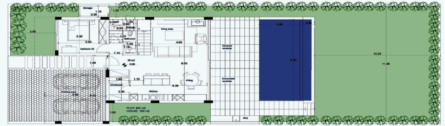
GROUND FLOOR
