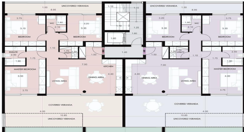
Typical layout Block A and B
