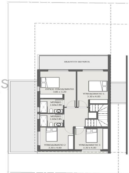
FLOOR PLANS - FIRST FLOOR
