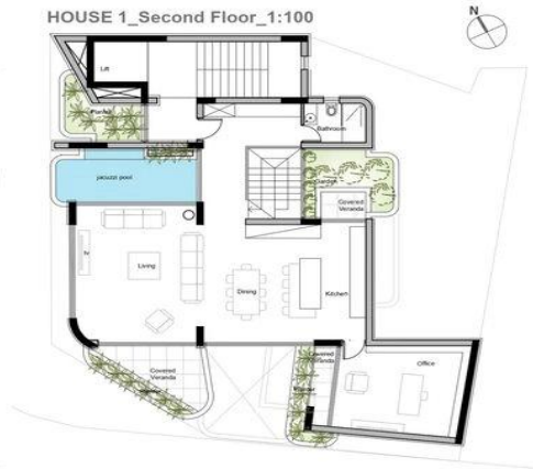
HOUSE 1_Second Floor_1:100
