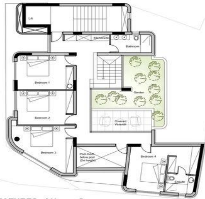
HOUSE 2_Third Floor_1:100
