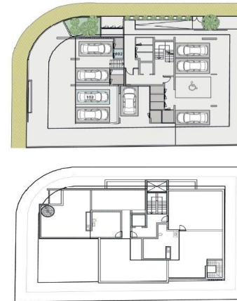
102 1 BEDROOM INDOOR AREA: 50.5 m 2 COVERED VERANDA: 14.8 m 2 + PLANTER: 4.3 m 2 STORAGE ROOM: 2.7 m 2 PARKING LOT: 1
