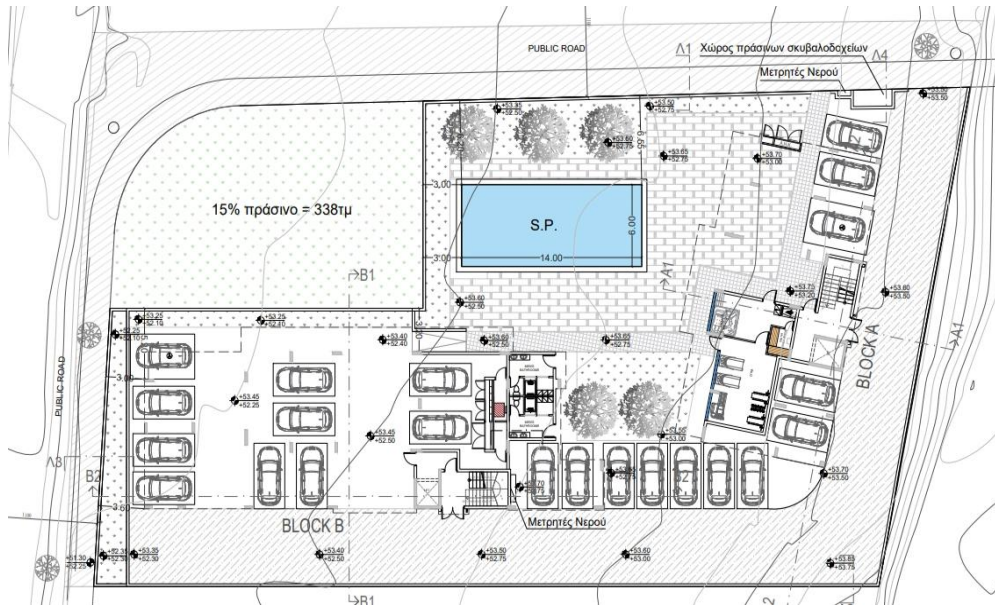
Floor Plan
