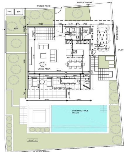
VILLA 13 PLOT AREA 381 SQM GROUND FLOOR BUILT AREA 74 SQM COVERED VERANDA 23 SQM COVERED PARKING AREA 20 SQM PLANT ROOM 9 SQM FIRST FLOOR BUILT AREA 91 SQM COVERED VERANDA 5 SQM
