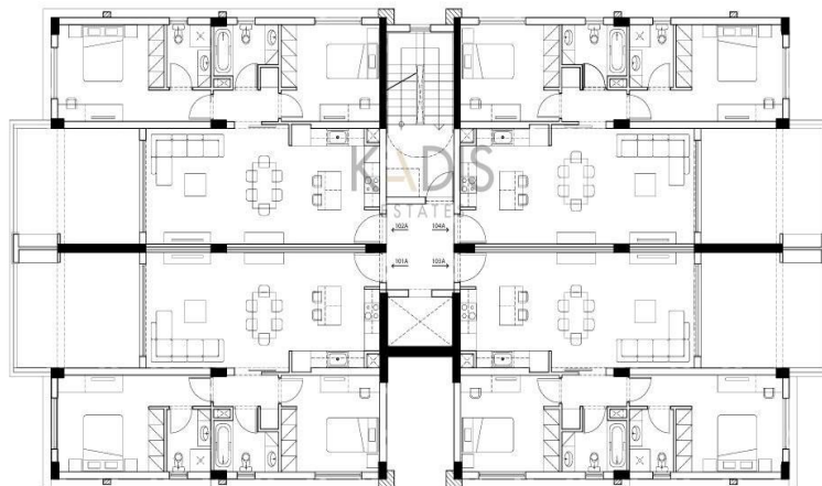
Apartment plan First Floor Block A
