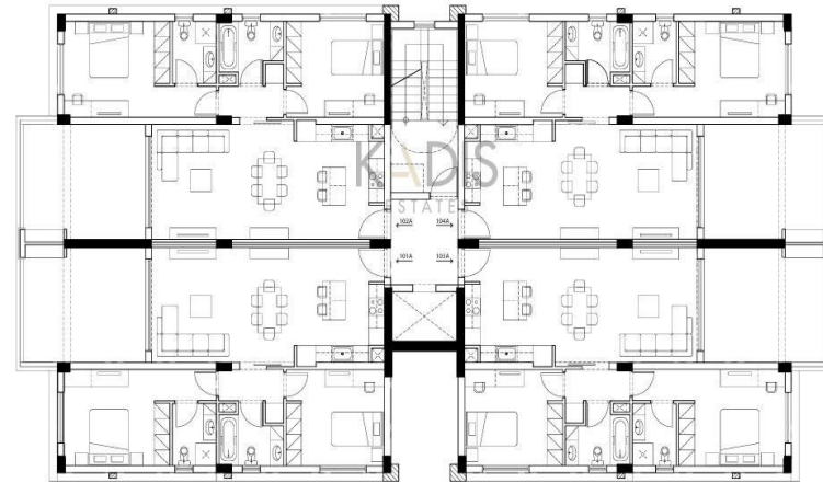
Apartment plan Second Floor Block A
