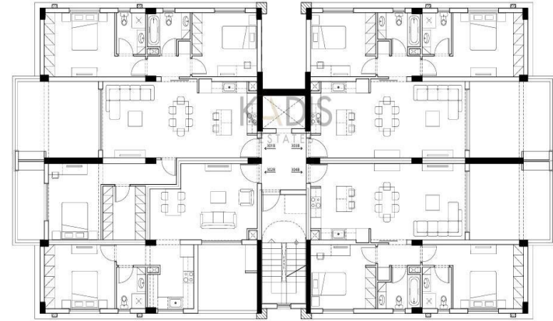
Apartment plan Third Floor Block B
