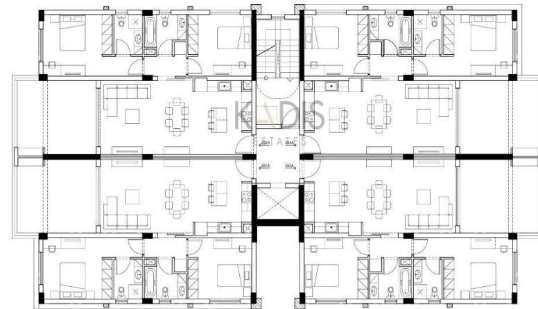
Apartment plan Second Floor Block A
