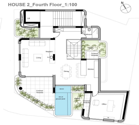
HOUSE 2_Fourth Floor_1:100
