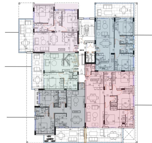
FLOORPLANS – SECOND FLOOR
