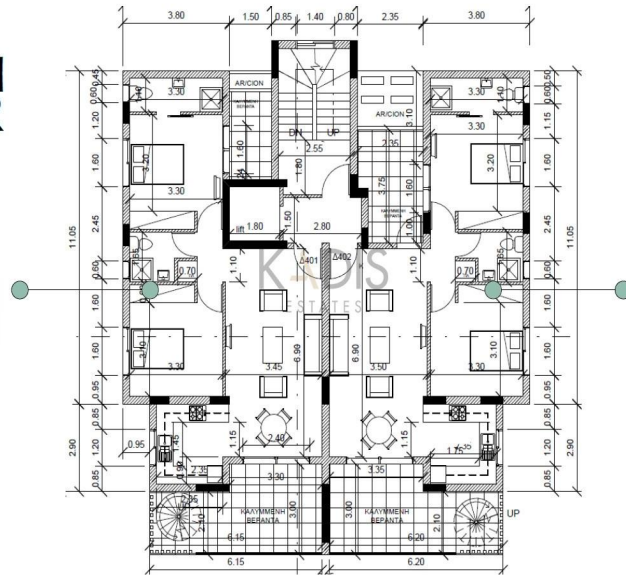
FLOORPLANS FORTH FLOOR
