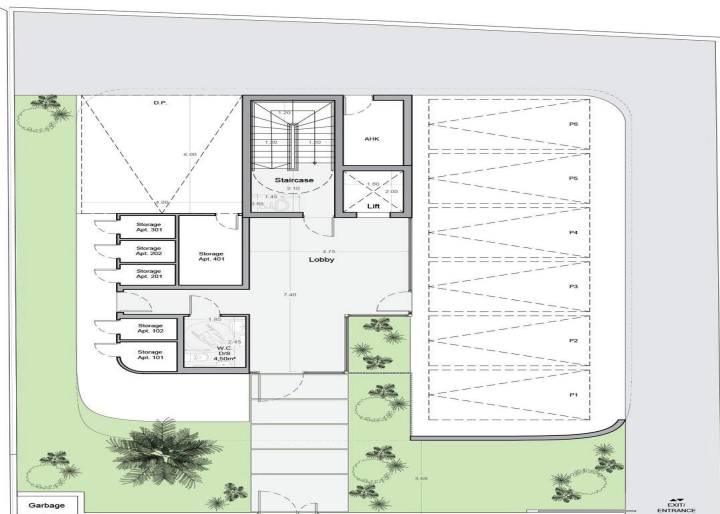
Ground FLOOR PLANS
