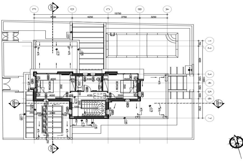
HOUSE CAMELIA - FIRST FLOOR PLAN SCALE 1:100 01/2003
