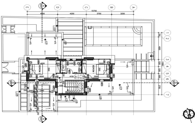
HOUSE CAMELIA - FIRST FLOOR PLAN SCALE 1:100 01/1000
