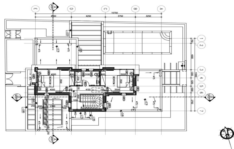
HOUSE CAMELIA - FIRST FLOOR PLAN (01) SCALE 1:100 (A003)
