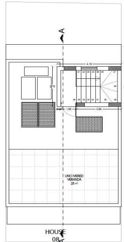
ROOF PLAN
