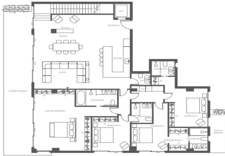
SEVENTH FLOOR
