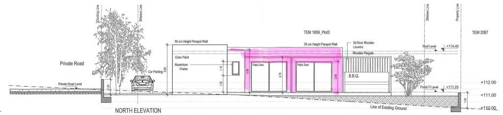
NORTH ELEVATION
