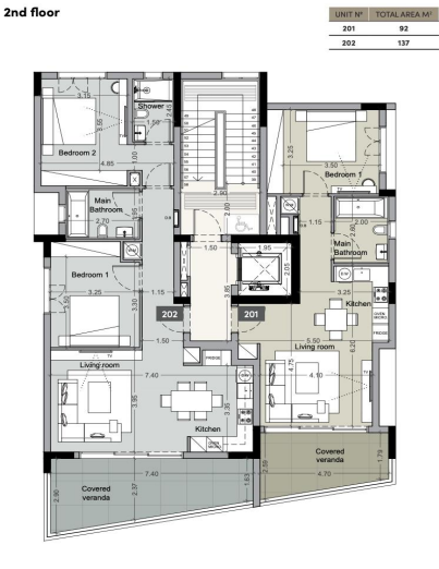
⌋ floor plans 2nd floor
