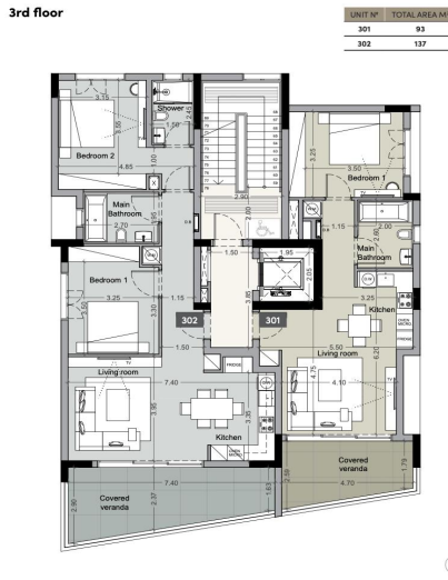
⌋ floor plans 3rd floor
