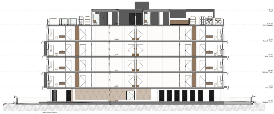
S-02 Section B-B
