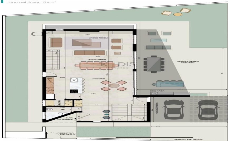
Ground Floor Internal Area: 124m 2
