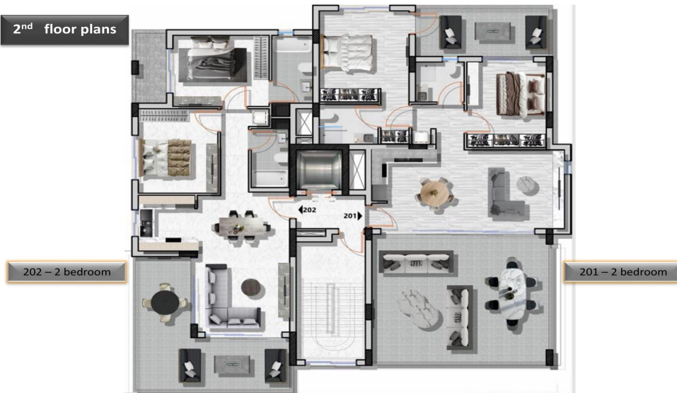
2 ND FLOOR PLANS – 2-BEDROOM APARTMENTS
