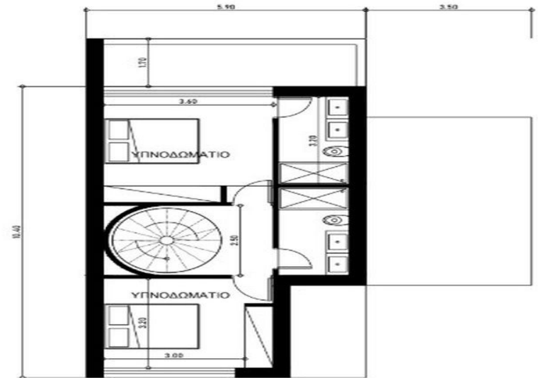
BASEMENT FLOOR: 62 m 2
