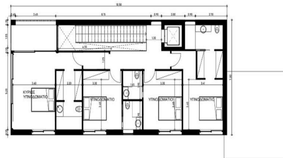
FIRST FLOOR: 130 m 2
