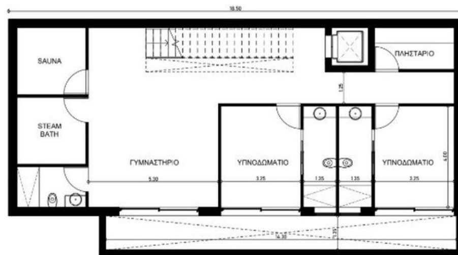
BASEMENT FLOOR: 170 m 2
