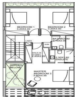
FIRST FLOOR PLAN SCALE 1:100
