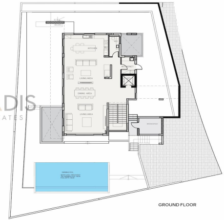
The View Phase B-Villa 1 Floor Plans
