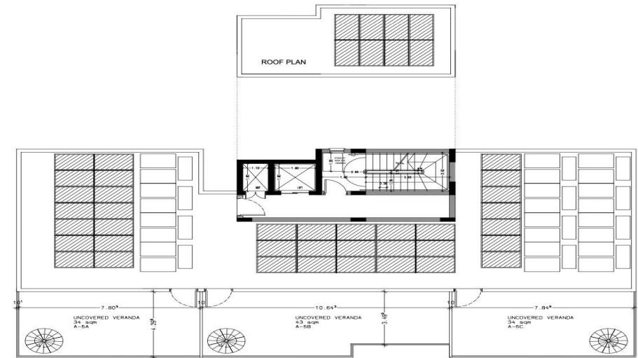
ROOF PLAN BLOCKS A,C,D,E,F,G 1st, 2nd, 3rd, 4th, 5th FLOORS
