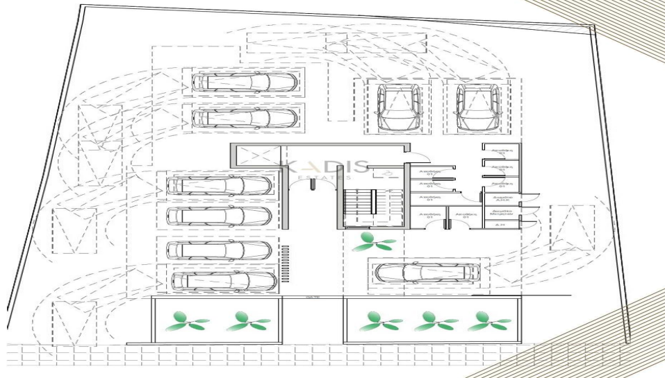
Architectural plans Ground Level
