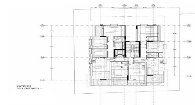
3RD FLOOR
