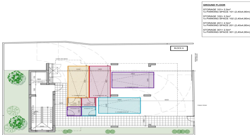
BLOCK A SITE PLAN - GROUND FLOOR SCALE 1:100
