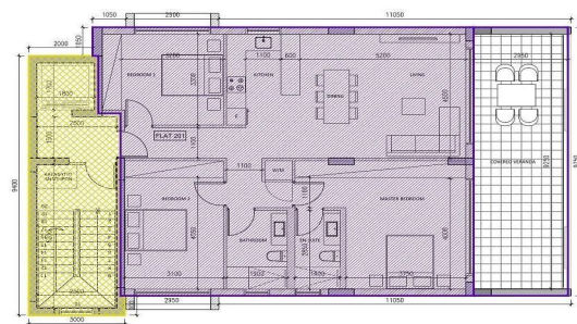
BLOCK A SECOND FLOOR SCALE 1:100
