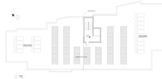
Roof 1:100
