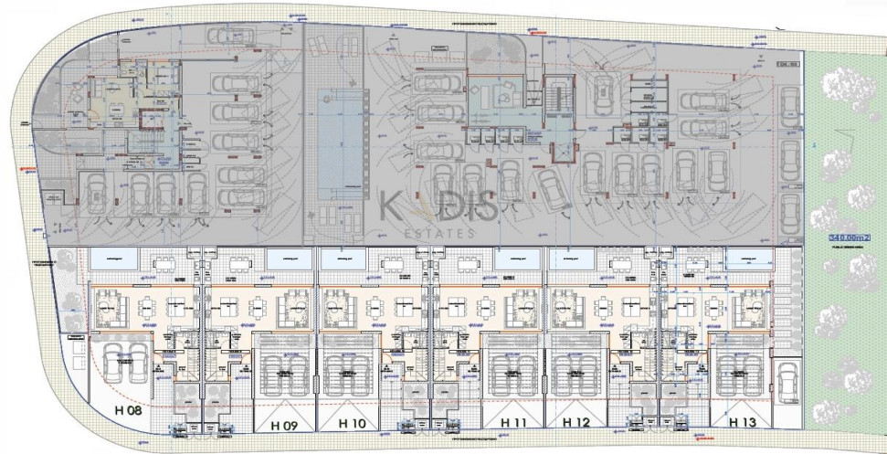
HOUSES - GROUND FLOOR
