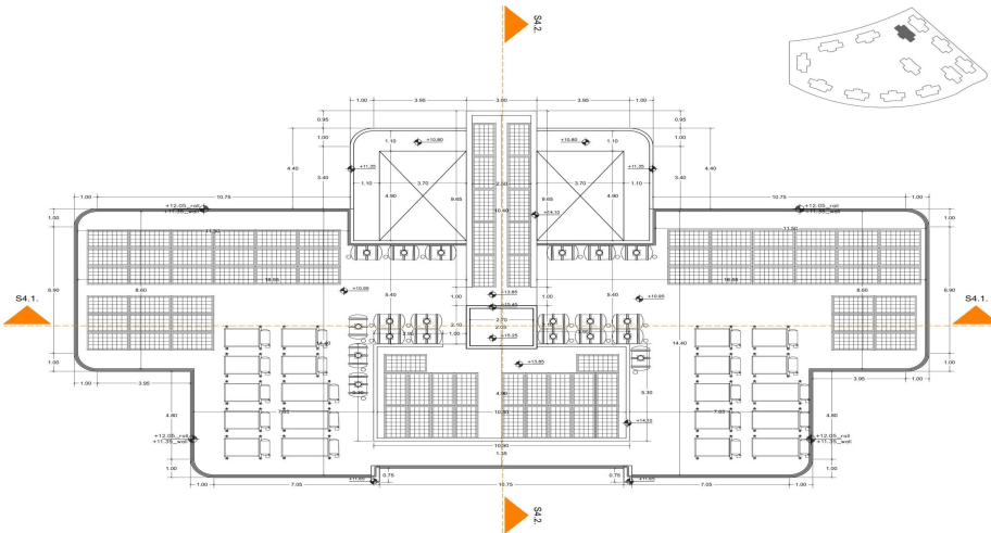
ROOF
