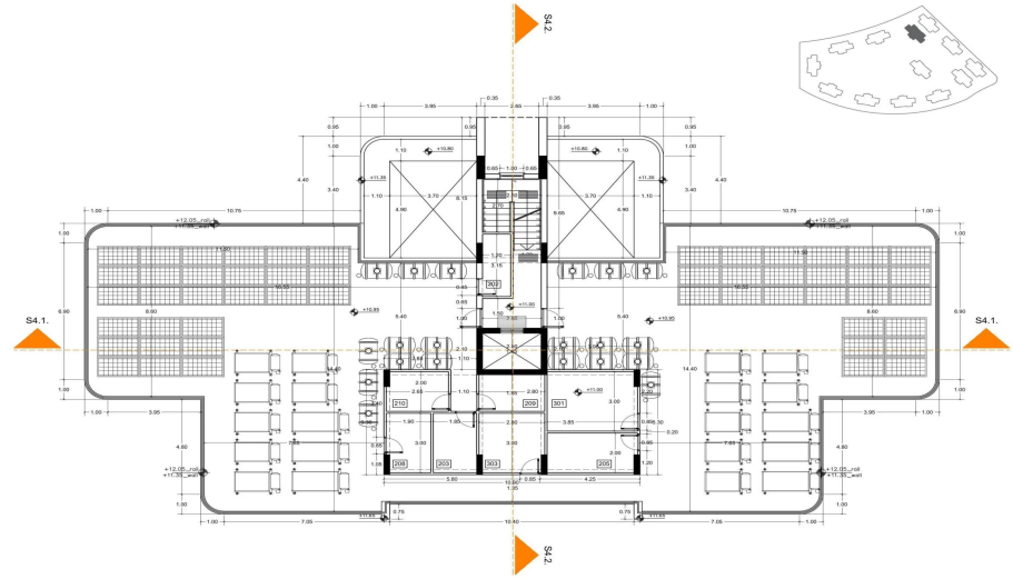
ROOF PLAN
