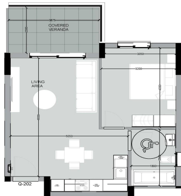
apartment Q - 202 layout plan
