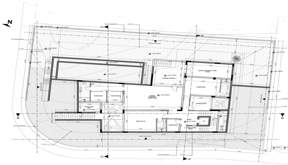
BASEMENT PLAN
