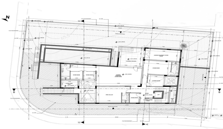
BASEMENT PLAN
