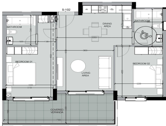
apartment S - 102 layout plan
