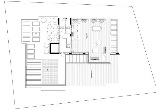
Roof Garden Plan
