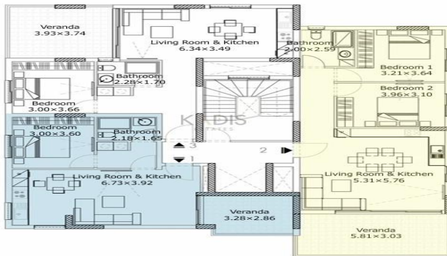
FIRST & SECOND FLOORS' PLAN
