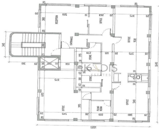
6th FLOOR
