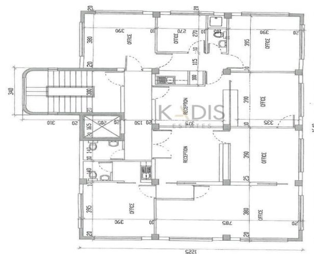
2nd FLOOR
