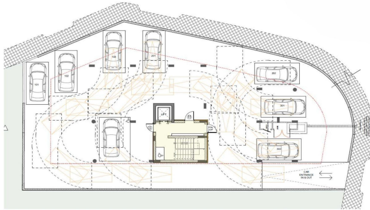
BASEMENT
