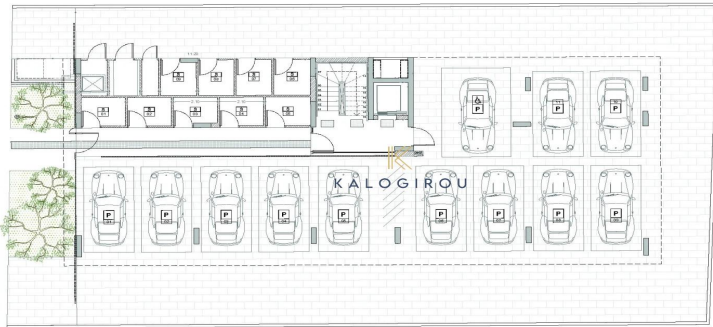
ODE RESIDENCE - GROUND FLOOR
