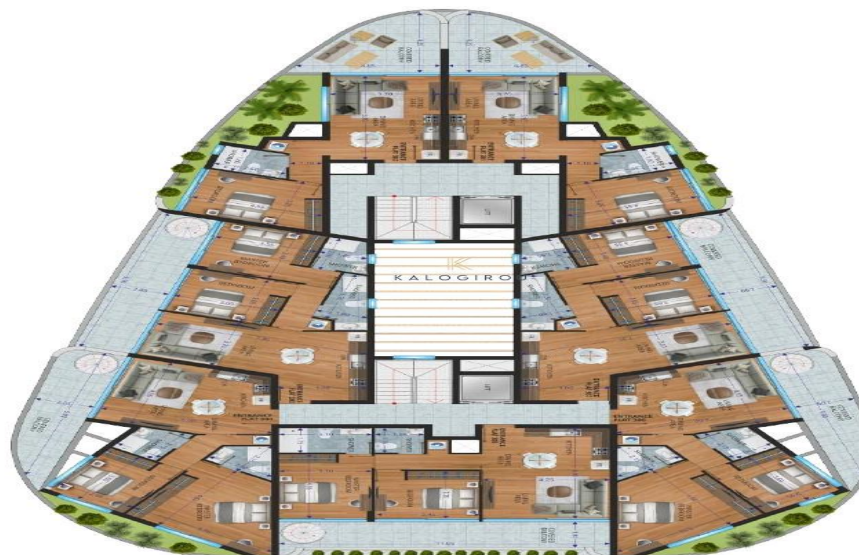
FLOOR PLANS
