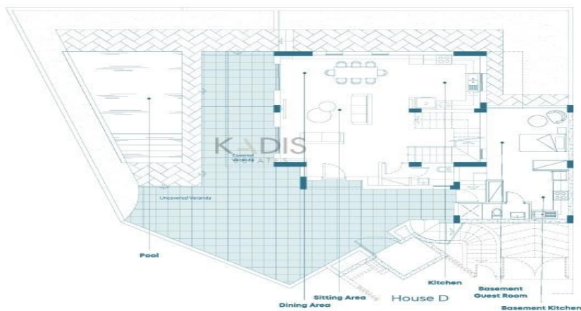
GROUND FLOOR Covered internal: 78 m 2 , Covered verandas: 16 m 2 Basement covered internal: 36 m 2
