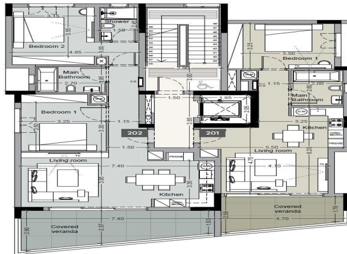
2nd floor
