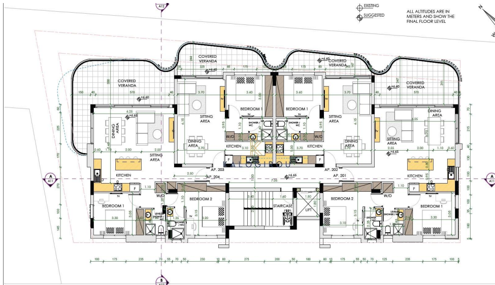
SECOND FLOOR PLAN 1:200
