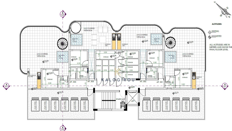
GARDEN ROOF PLAN 1:200
