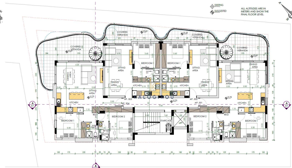
THIRD FLOOR PLAN 1:200
